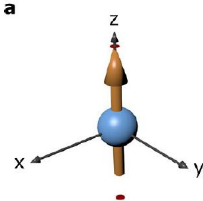
n=1 (1D-Ising)
