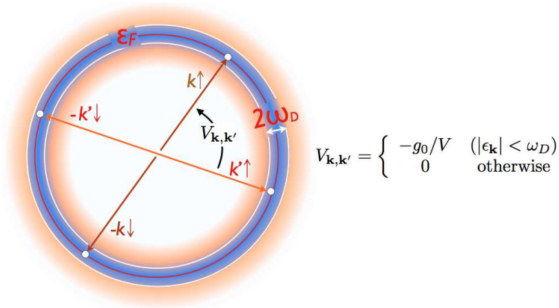
Fig. 14.6 In the BCS Hamiltonian, the matrix V_{\mathbf{k},\mathbf{k}'} acts attractively on pairs of electrons within \omega_D of the Fermi surface. Provided the repulsive interaction at higher energies is not too large, a superconducting instability results.
