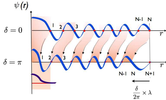
Fig. 15.5 Illustrating the Friedel sum rule. As the scattering phase shift grows, the nodes of the eigenstates at the Fermi surface are drawn into the potential well. Each time the phase shift passes through \pi one more node passes into the well, leading to one more bound-electron.
