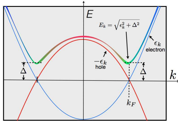
Fig. 14.7 Illustrating the excitation spectrum of a superconductor. Andreev scattering resulting scattering mixes the electron excitation spectrum (blue) with the hole excitation spectrum (red) producing the gap \Delta in the quasiparticle excitation spectrum. The quasiparticles at the Fermi momentum are linear combinations of electrons and holes, with an indefinite charge.
