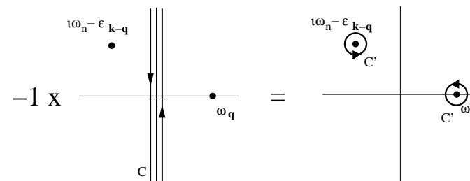
Fig. 9.5 Contours C and C' used in evaluation of \Sigma(\mathbf{k}, i\omega_n)
