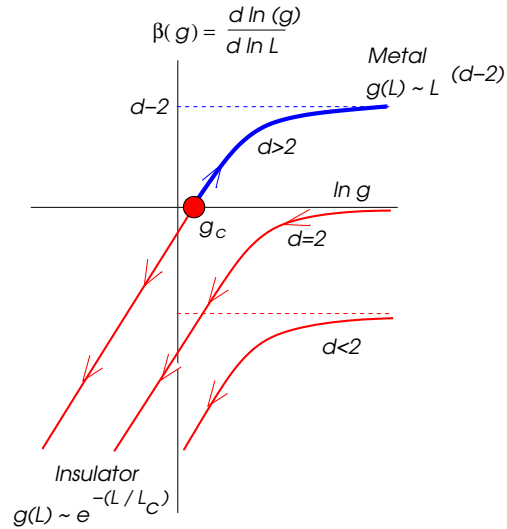
Fig. 11.6 The scaling function \beta(g) deduced by Abrahams et al. for a non-interacting metal. For d > 2 there is critical conductance g_c which gives rise to a disorder-driven metal-insulator transition. In d \leq 2 , disorder always gives rise to localization and the formation of an insulator.
