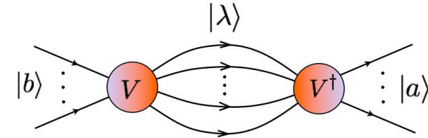
Fig. 15.13 T-matrix representation of interaction induced between states |b\rangle and |a\rangle by integrating out the virtual fluctuations into the high-energy states |\lambda\rangle .
