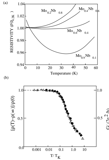
Fig. 15.17 (a) Sketch of resistance minimum in \text{Mo}_x\text{Nb}_{1-x} (b) Sketch of excess resistivity associated with scattering from an impurity spin. Right hand-scale- differential conductivity of a quantum dot.
