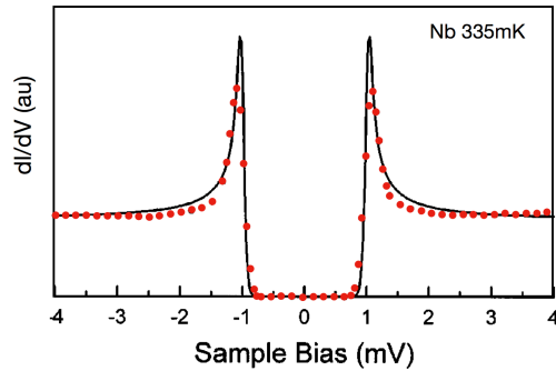
Fig. 14.13 Comparison between the experimental tunneling spectrum and the BCS spectrum, after Eric Hudson et al [21]
