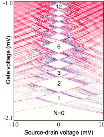
Fig. 15.8 Experimentally measured conductance for a voltage-biased quantum dot after [?], showing the splitting of the Coulomb blockade into two components, shifted up and down by the voltage bias, \pm eV_{sd}/2 . In the white diamond-shaped regions, G(V_{sd}) \approx 0 as a result of Coulomb blockade. The number of particles N is fixed in each of the diamond regions. The lines outside the diamonds, running parallel to the sides, identify excited states.
