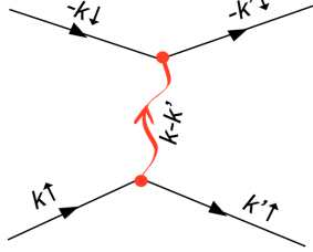
Fig. 14.4 Phonon exchange process responsible for the BCS interaction.
