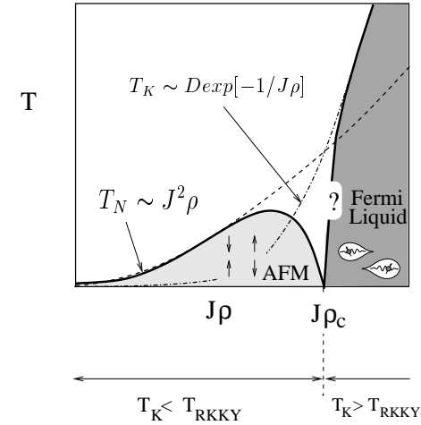
Fig. 16.3 Doniach diagram, illustrating the antiferromagnetic regime, where T_K < T_{RKKY} and the heavy fermion regime, where T_K > T_{RKKY} . Experiment has told us in recent times that the transition between these two regimes is a quantum critical point. The effective Fermi temperature of the heavy Fermi liquid is indicated as a solid line. Circumstantial experimental evidence suggests that this scale drops to zero at the antiferromagnetic quantum critical point, but this is still a matter of controversy.
