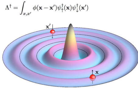
Fig. 14.3 Illustration of a “Cooper pair”. (Note: the location of the electrons relative to the pair wavefunction involves artistic license since the wavefunction describes the relative position of the two electrons.)
