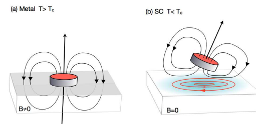
Fig. 14.1 (a) A magnet rests on top of a normal metal, with its field lines penetrating the metal. (b) once cooled beneath T_c , the superconductor spontaneously excludes magnetic fields, generating persistent supercurrents at its surface causing the magnet to levitate.
