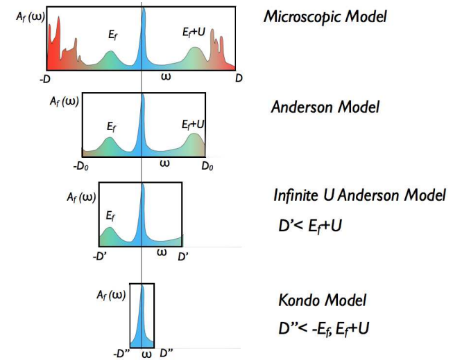
Fig. 15.12 Scaling concept. Low energy model Hamiltonians are obtained from the detailed original model by integrating out the high energy degrees of freedom. At each stage, the physics described by the model spans a successively lower frequency window in the excitation spectrum.
