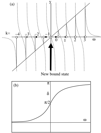
Fig. 16.6 (a) Graphical solution of the equation y = -\sum_k \frac{V_o^2}{y - \epsilon_k} , for eight equally spaced conduction electron energies. Notice how the introduction of a new bound-state at y = 0 displaces electron band-states both up and down in energy. In this way, the Kondo effect injects new bound-state fermion states into the conduction sea. (b) Energy dependence of the scattering phase shift.
