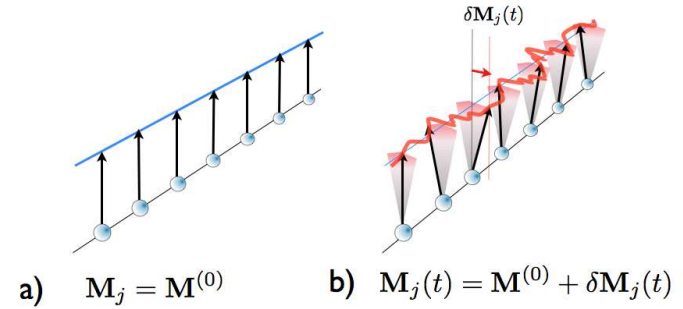
Fig. 13.7 Illustrating (a) mean-field theory (b) fluctuations about mean-field theory.
