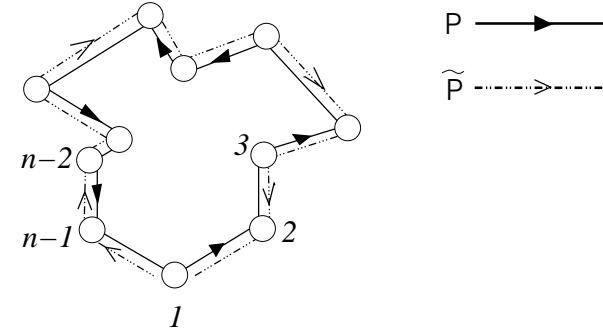
Fig. 11.3 Scattering of an electron around two time-reversed paths
