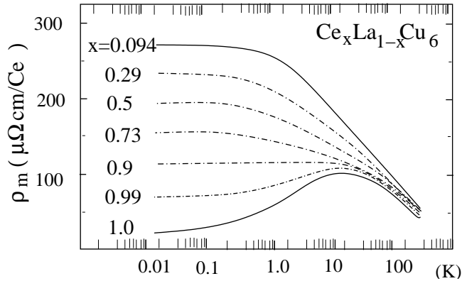
Fig. 16.4 Development of coherence in heavy fermion systems. Resistance in Ce_{1-x}La_xCu_6 after Onuki and Komatsubara[?]
