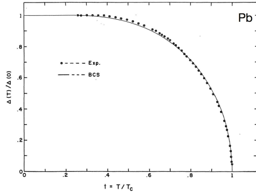
Fig. 14.11 Comparing the temperature dependence of the gap on the reduced temperature T/T_c with the gap measured by tunneling in superconducting lead, after [20].
