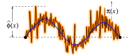
Quantum string.
