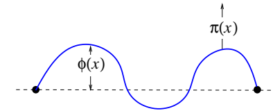
Classical string.
