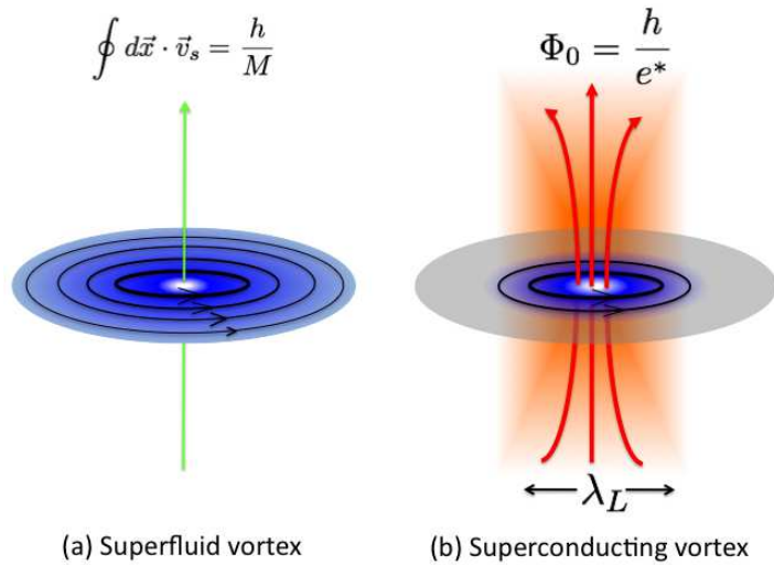
Fig. 12.10 Contrasting (a) a vortex in a neutral superfluid with (b) a vortex in a superconductor, where each unit of quantized circulation binds one quanta of magnetic flux.
