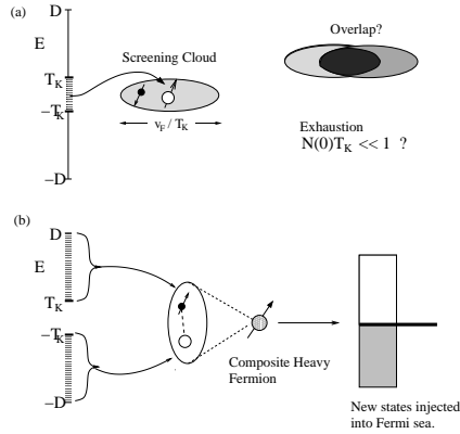
Fig. 16.5 Contrasting (a) the “screening cloud” picture of the Kondo effect with (b) the composite fermion picture. In (a), low energy electrons form the Kondo singlet, leading to the exhaustion problem. In (b) the composite heavy electron is a highly localized bound-state between local moments and high energy electrons which injects new electronic states into the conduction sea at the chemical potential. Hybridization of these states with conduction electrons produces a singlet ground-state, forming a Kondo resonance in the single impurity, and a coherent heavy electron band in the Kondo lattice.
