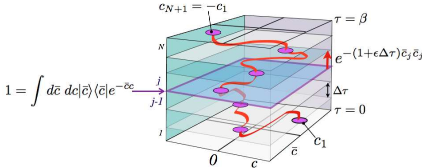
Division of Grassmanian time evolution into "time-slices".
