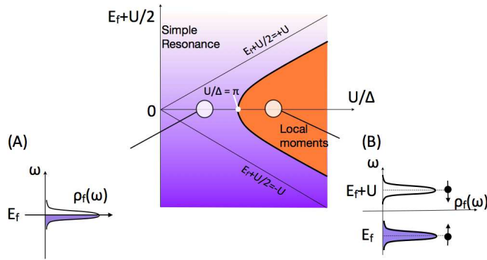
Fig. 15.6 Mean field phase diagram of the Anderson model, illustrating how the f-electron resonance splits to form a local moment. A) U < \pi\Delta , single half-filled resonance. B) U > \pi\Delta , up and down components of the resonance are split by an energy U .
