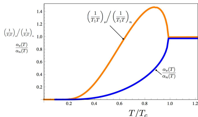
Fig. 14.14 Showing the effect of coherence factors NMR and ultrasonic attenuation in a superconductor, calculated in BCS theory. Orange line displays the NMR relaxation rate, showing the Hebel Slichter peak. Blue line, the ultrasound attenuation. The integrals entering the NMR relaxation rate are formally divergent for T < T_c and were regulated by introducing a small imaginary damping rate i\delta to the frequency where \delta/\Delta = 0.005 .
