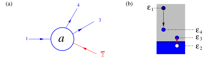
Fig. 7.7 Decay of a quasiparticle into two quasiparticles and a quasihole. (a) Scattering process. (b) Energies of final states.
