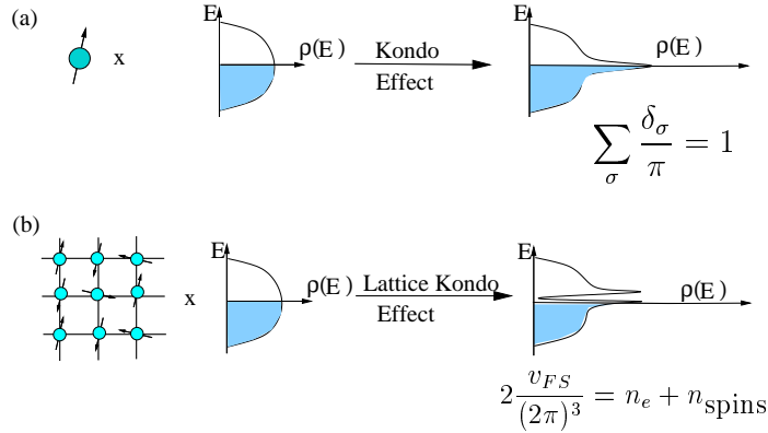
Fig. 16.2 (a) Single impurity Kondo effect builds a single fermionic level into the conduction sea, which gives rise to a resonance in the conduction electron density of states (b) Lattice Kondo effect builds a fermionic resonance into the conduction sea in each unit cell. The elastic scattering off this lattice of resonances leads to formation of a heavy electron band, of width T_K .
