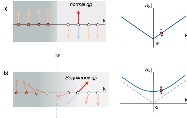
Fig. 14.9 Illustrating how the excitation of quasiparticle pairs corresponds to an “isospin flip”, which forms a pair of up and down quasiparticles with energy 2|B_k| . (a) Quasiparticle pair formation in the normal state where the quasiparticle spectrum is gapless (b) formation of a “Boguilubov” quasiparticle pair in the superconducting state where the excitation spectrum is gapped
