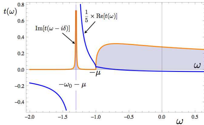
Fig. 8.4 Showing real and imaginary parts of the t-matrix function for scattering off an attractive delta function potential in two dimensions. The bound-state at \omega = -\omega_o - \mu develops for arbitrarily small attractive interaction in two dimensions
