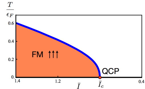
Fig. 13.6 Phase diagram for 3D “Stoner model” computed using (13.213) and (13.214). The horizontal axis is the coupling constant \bar{I} = I N(0) , where the critical value \bar{I}_c = 1 .
