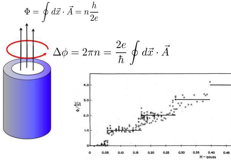
Fig. 12.11 Flux quantization inside a cylinder. In the lowest energy configuration, with no supercurrent in the cylinder walls, the \Delta\phi = 2\pi n twist in the phase of the order parameter around the cylinder is compensated by a quantized circulation of the vector potential, giving rise to a quantized flux. The inset shows quantized flux measured in reference [16].
