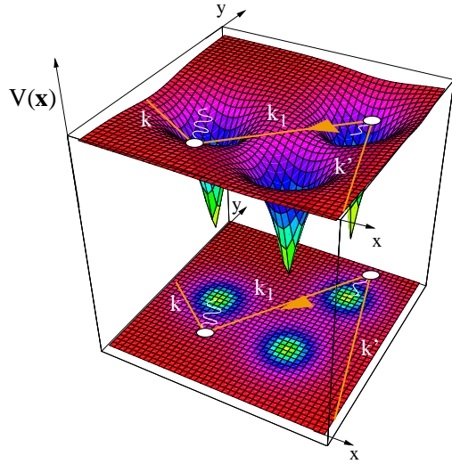
Fig. 9.4 Double scattering event in the random impurity potential.
