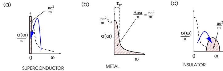
Fig. 10.3 The f-sum rule. Illustrating (a) the spectral weight transfer down to the condensate in a superconductor (b) the Drude weight in a simple metal and (c) The spectral weight transfer up to the conduction band in an insulator. )
