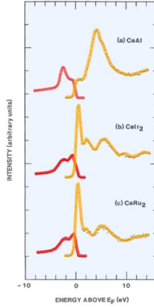
Fig. 15.11 Spectral functions for three different Cerium f-electron materials, measured using X-ray photoemission (below the Fermi energy) and inverse X-ray photoemission (above the Fermi energy) after [?]. CeAl is an antiferromagnet and does not display a Kondo resonance.
