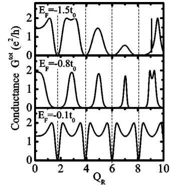
FIG. 3. The total conductance G^{\text{tot}}(Q_R, E_F) of a strictly 1D ring (M,N)=(1,200) , attached to two 1D semi-infinite ideal leads, as a function of dimensionless Rashba SO coupling Q_R=t_{\text{so}}N/t_0\pi , for three different values of the Fermi energy as a parameter. The vertical dotted lines denote the position of the conductance minima G^{\text{tot}} \approx 0 , which do not depend on E_F at which the zero-temperature quantum transport takes place.
