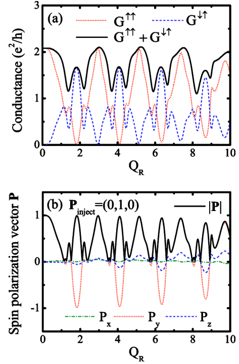
FIG. 8. (Color online) The spin-resolved conductances (a) G^{\sigma\sigma'}(Q_R, E_F) and the outgoing current spin polarization vector (b) \mathbf{P}(Q_R, E_F) vs the Rashba SO interaction Q_R = t_{\text{so}}N/t_0\pi for a finite-width conductor with (M, N) = (3, 200) and Fermi energy E_F = -0.1t_0 . The spin-quantization axis is chosen to be the y -axis.
