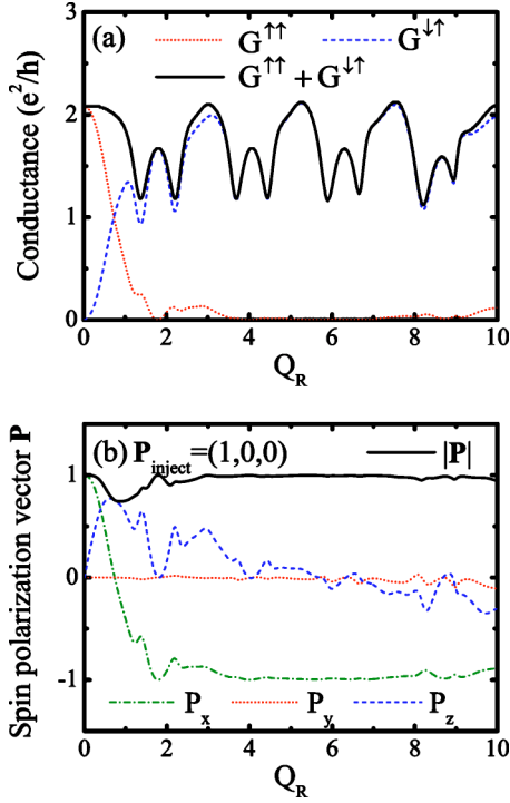
FIG. 7. (Color online) The spin-resolved conductances (a) G^{\sigma\sigma'}(Q_R, E_F) and the outgoing current spin polarization vector (b) \mathbf{P}(Q_R, E_F) vs the Rashba SO interaction Q_R = t_{\text{so}}N/t_0\pi for a finite-width conductor with (M, N) = (3, 200) and Fermi energy E_F = -0.1t_0 . The spin-quantization axis is chosen to be the x -axis.
